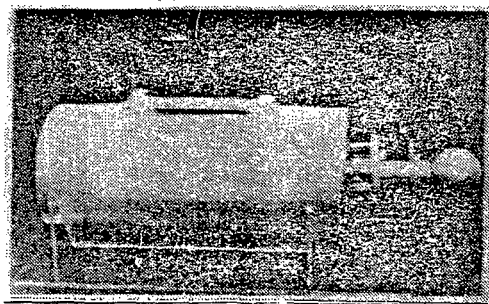
Figure 2. Photograph of Spiral Generator Prior to Impregnation with Castor Oil. The Input Gas-Dielectric; Rail Switch is 1 ft Long.
